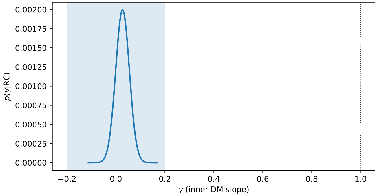
RC-only posterior for inner slope \gamma (gNFW halo + GP)
