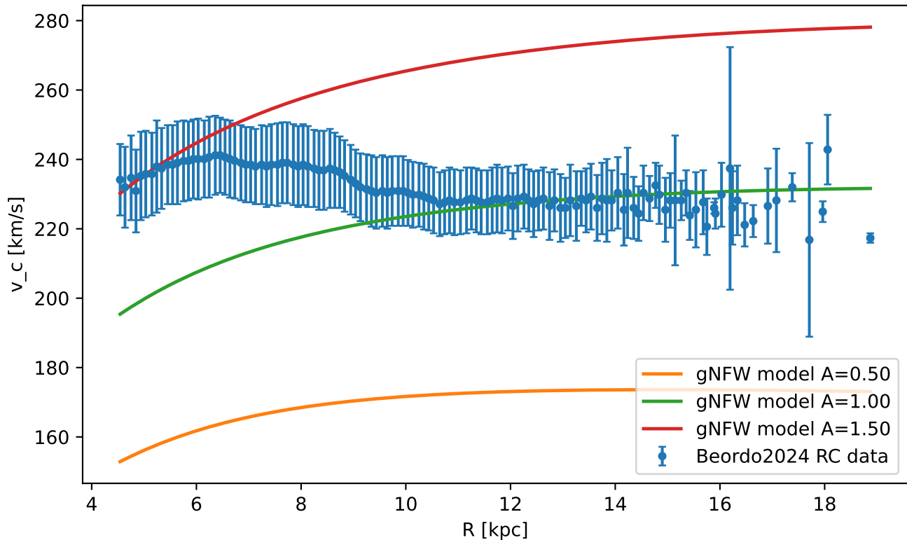
Rotation curve test for spherical gNFW halo (gamma free, A scaling)
