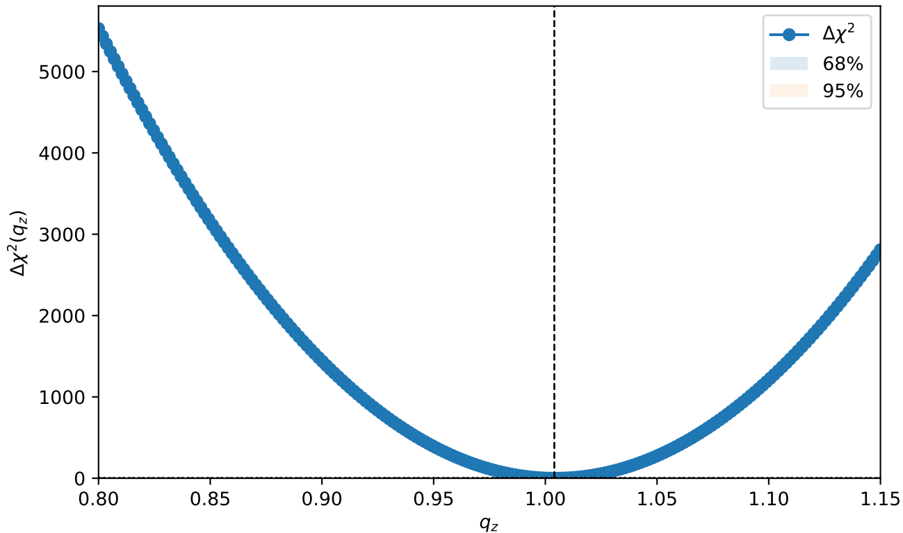
GD-1 + rotation curve proxy for q_z (offset+slope, robust)
