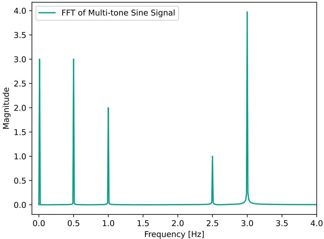
FFT of Multi-tone Sine Signal
