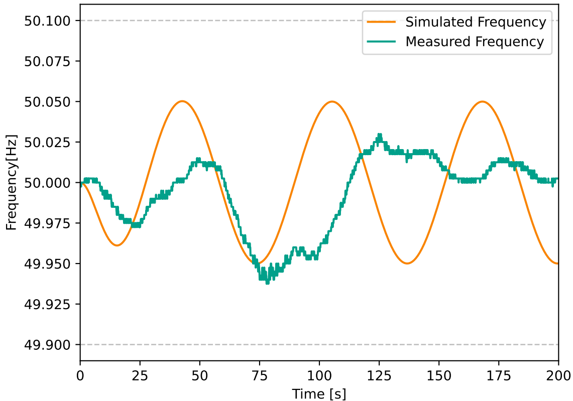
Grid Frequency
