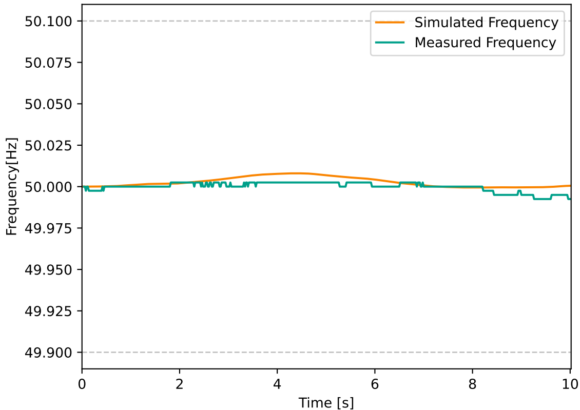
Grid Frequency
