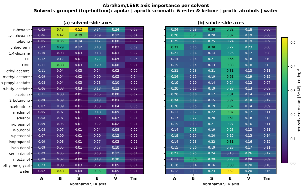
Figure 26: Abraham/LSER axis importance per solvent. Rows are solvents grouped (top-bottom) into apolar, aprotic-aromatic + ester / ketone, protic alcohols, and water. Columns are the six Abraham/LSER axes. Cells are mean(|SHAP|) for that (side, solvent, axis) cell on eval. The panel reads as a literal LSER table: alkanes have very large B and S on the solvent side (the model uses the absence of those features to identify the medium), water has a large solvent-side E and the largest solute-side E in the dataset, and DMF/toluene foreground solvent-side B .
