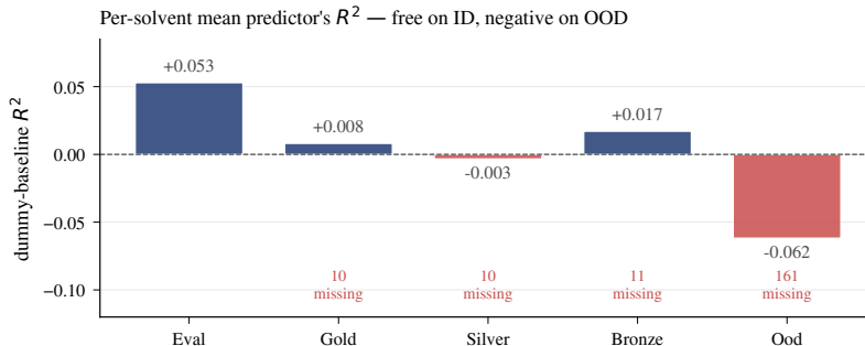
Figure 10: Per-solvent-mean predictor’s R^2 across the five evaluation splits. Positive on in-distribution Eval, near-zero on tiers, and negative on OOD (161 solvents unseen during training, so the predictor falls back to the grand mean). Motivates a metric suite in which aggregate R^2 or RMSE does not reward solvent identification.
