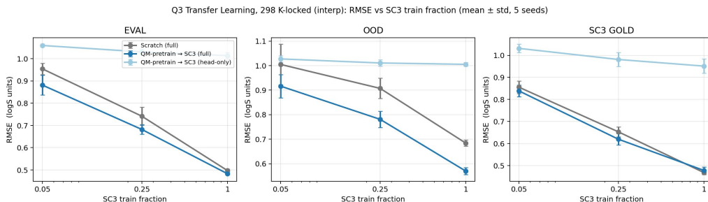
Figure 18: 298 K-locked transfer (Apelblat-evaluated at T = 298.15 K). RMSE on eval (left), ood (middle), and sc3_gold (right) as a function of SC 3 -train fraction. Mean \pm std over 5 seeds. The QM-pretrained model (blue) wins in 8 of 9 cells; the only non-win is sc3_gold at 100% data, where scratch and QM are tied within 1\sigma .
