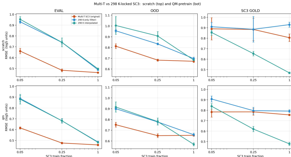
Figure 19: Multi-T vs. 298 K-locked, side-by-side. Same 5-seed runs as Tables 15 and 16. Top row: scratch. Bottom row: QM. At 100% SC 3 -train, the single-T sc3_gold RMSE is roughly half the multi-T value, with QM-pretraining and scratch converging — the residual error budget at room temperature is dominated by aleatoric noise rather than missing chemistry signal. (The FILTER curves shown in the figure are an alternative single-T construction that keeps only real measurements with T \in [295.15, 301.15] K; we use the Apelblat-evaluated variant in the main text because its larger training set avoids overfitting.)
