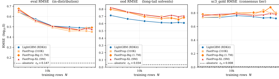
Figure 13: Test RMSE vs. training-set fraction for representative models (seven fractions \times fixed seeds).
