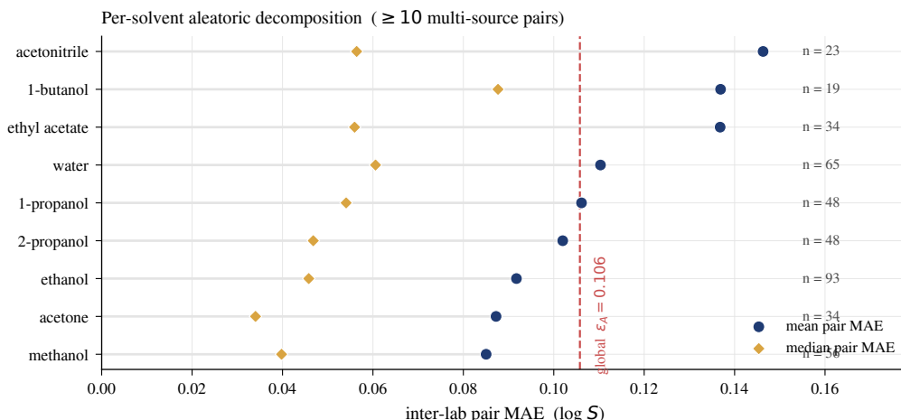
Figure 5: Per-solvent aleatoric decomposition (primary, HoS-excluded, solvents with \geq 10 multi-source pairs). Lollipops are mean pair MAE; diamonds are median; n is the multi-source pair count. Dashed vertical line is the global \epsilon_{\text{aleatoric}} = 0.106 .
