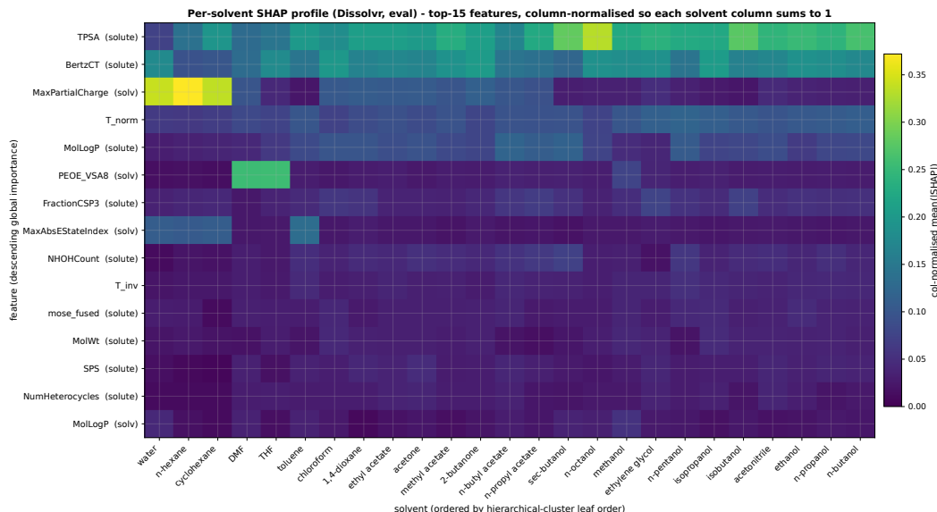
Figure 23: Per-solvent SHAP profile (Dissolvr, eval) . Rows are the top-15 globally-important features (descending); columns are the 25 eval solvents, ordered by hierarchical clustering on the column vectors. Cells are column-normalised mean(|SHAP|), so darker = less important relative to the rest of that solvent’s profile. Two qualitative patterns are visible: (i) for typical organic solvents the model relies on TPSA and BertzCT of the solute ; (ii) for the extreme solvents (water, n-hexane, cyclohexane) it switches to MaxPartialCharge and MaxAbsEStateIndex of the solvent . A third specialised pattern shows up for DMF and THF, where PEOE_VSA8 of the solvent dominates.
