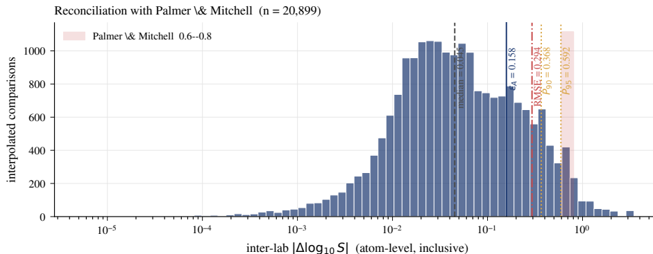
Figure 6: Reconciliation with Palmer and Mitchell [2014]. The inclusive atom-level |\Delta \log_{10} S| distribution ( n = 20\,899 interpolated comparisons) is plotted on a log- x axis; vertical lines are our summary statistics. The shaded band is Palmer & Mitchell’s quoted 0.6–0.8 log S aqueous range, which coincides with our P_{90} – P_{95} and RMSE, not with the expected error.
