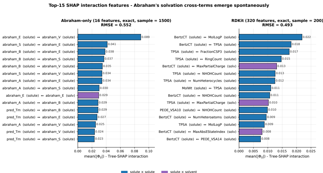
Figure 27: Top SHAP interaction features. Bars are \text{mean}(|\Phi_{ij}|) on eval; colour encodes the block-pair (solute×solute, solute×solvent, etc.). On Abraham-only, the top-8 pairs are exclusively within the solute LSER axes (textbook within-molecule solvation coupling); cross-block solute×solvent pairs appear from rank 9 onward and are matched-axis ( E \times E , A \times A , E \times B ) – the off-diagonal LSER cross-terms. On RDKit, the top-4 pairs are within the GSE axes (BertzCT×MolLogP, etc.); the largest cross-block interaction is BertzCT(solute) × MaxPartialCharge(solv), the discrete analogue of a partition coefficient term.
