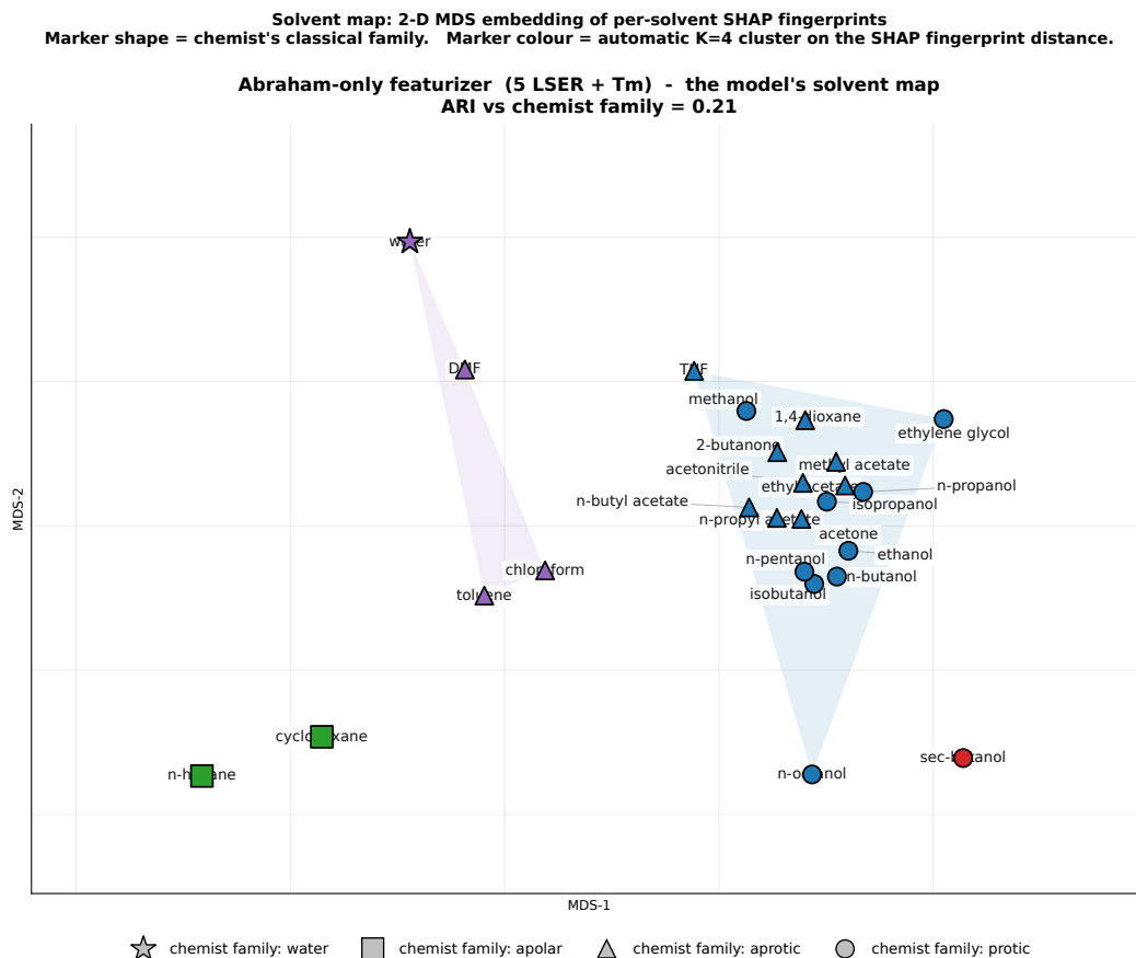
Figure 24: Solvent map under the Abraham-only featurizer. Each point is one of the 25 eval solvents at its 2-D MDS coordinates derived from the per-solvent SHAP fingerprint distance 1 - \cos(\cdot) . Marker shape encodes the chemist's classical Snyder family (☆ water, ■ apolar alkane, ▲ aprotic, ● protic alcohol). Marker colour encodes the model's automatic cluster (K=4 average-linkage hierarchical, on the same distance). Same colour = the model treats those solvents the same way; same shape = chemists treat them the same way. Disagreements – such as the model placing water in the same purple cluster as DMF / chloroform / toluene – are visually obvious. ARI vs the chemist labelling = 0.21.
