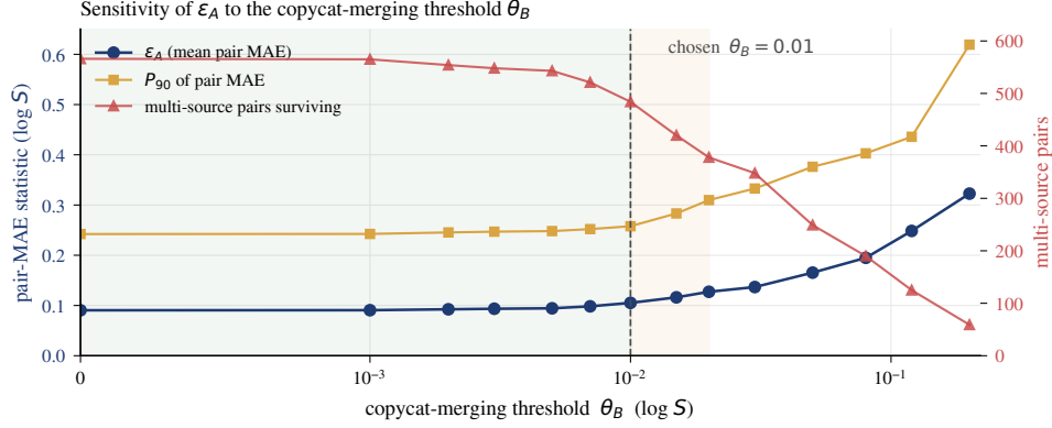
Figure 2: Sensitivity of \varepsilon_{\text{aleatoric}} and the multi-source pair count to the copycat-merging threshold \theta_B . The chosen value \theta_B = 0.01 (dashed line) sits at the upper edge of the shaded “safe” region, where each merged pair is a genuine copy. The shaded “cliff” region [0.01, 0.02] loses 106 multi-source pairs — more than the entire loss incurred between 0 and 0.01.
