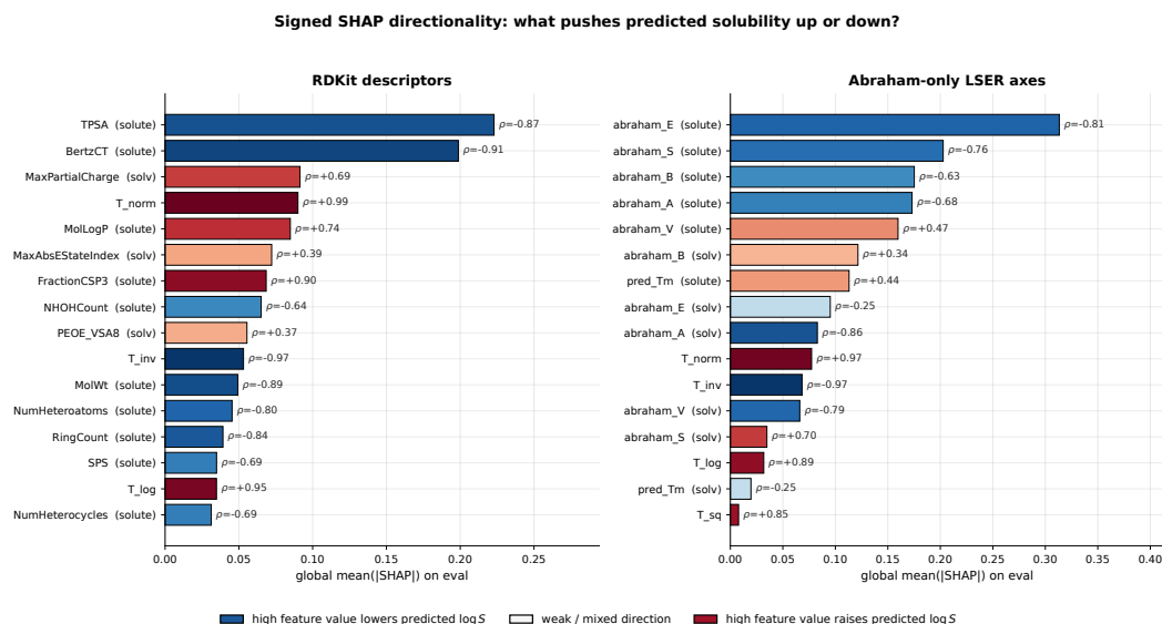
Figure 22: Signed SHAP directionality. Bar length is the usual global mean(|SHAP|), so the ranking is unchanged from Figure 21. Bar colour and the printed Spearman \rho show direction: blue features have high values that lower predicted \log_{10} S , red features have high values that raise predicted \log_{10} S . The descriptor panel says the strongest solute features – TPSA, BertzCT, MolWt, RingCount, heteroatom counts – mostly push predictions down when large, while temperature and solvent partial-charge features push predictions up. The Abraham-only panel makes the LSER story explicit: solute E, S, B, A lower predicted solubility when large, whereas increasing temperature raises it.
