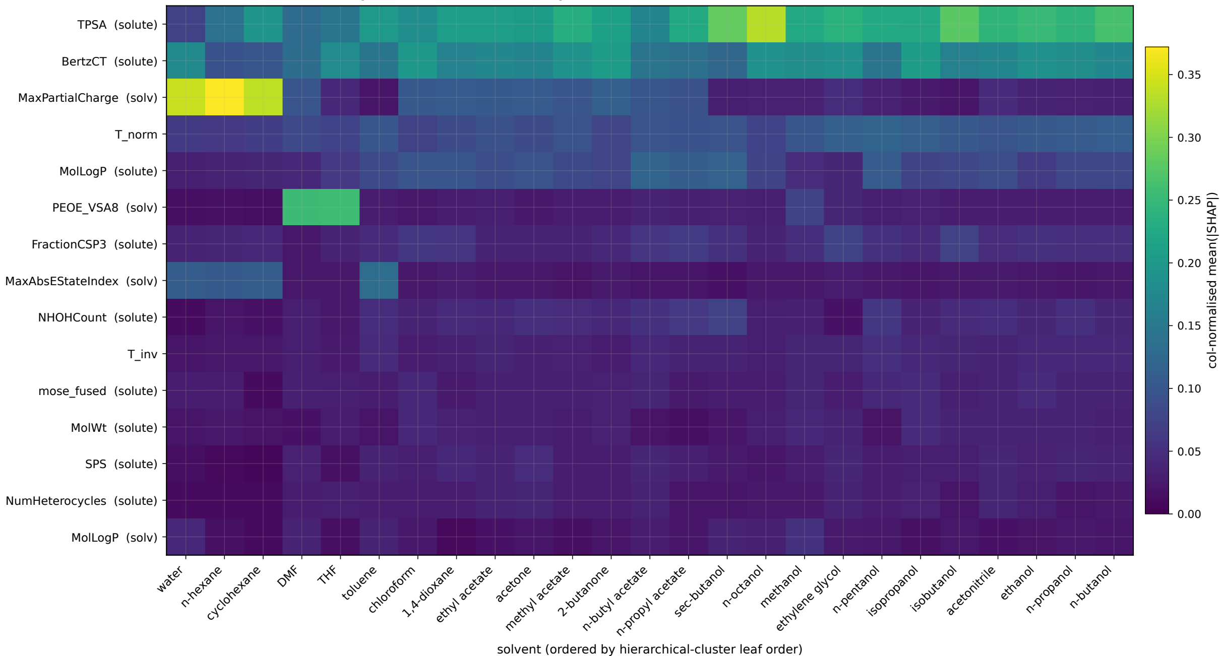
Per-solvent SHAP profile (Dissolvr, eval) - top-15 features, column-normalised so each solvent column sums to 1
