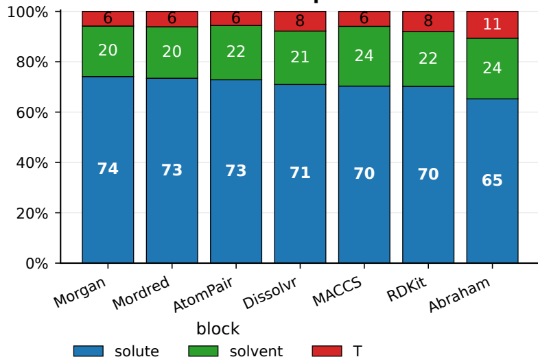
eval split
