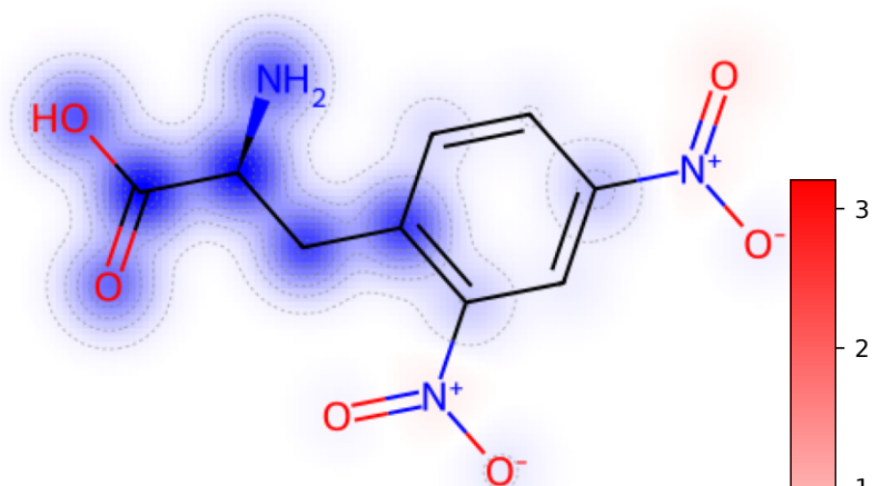
carboxylic acid solvent=ethyl acetate; pred=-3.96, y=-4.74
