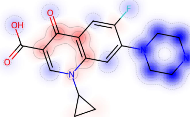
piperazine / diamine solvent=acetone; pred=-3.56, y=-3.90
