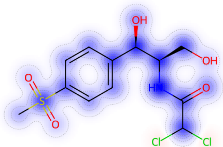
sulfur-rich / sulfone solvent=ethyl acetate; pred=-3.07, y=-3.19
