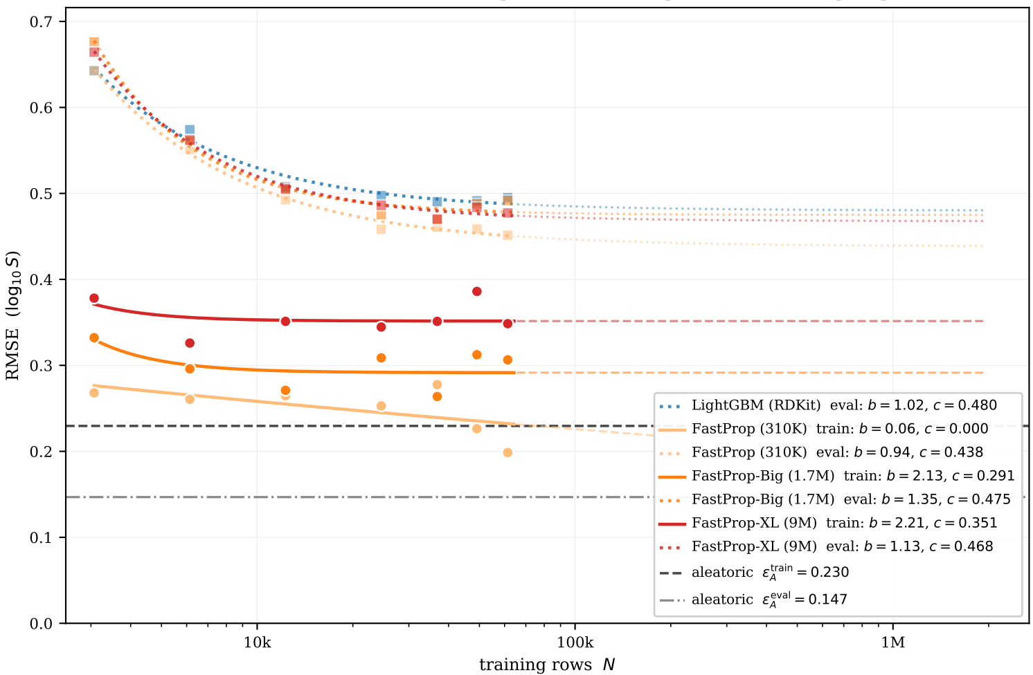
Train RMSE@best (circles, solid) vs. eval RMSE (squares, dotted) -- power-law fits and per-split aleatoric floors
