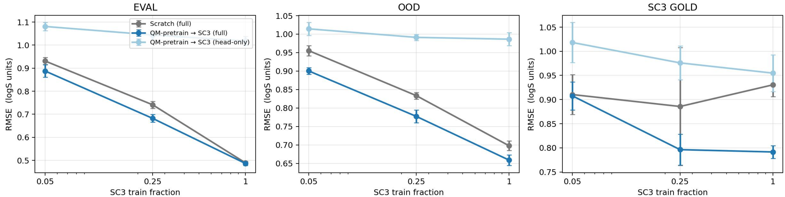
Q3 Transfer Learning, 298 K-locked (filter): RMSE vs SC3 train fraction (mean \pm std, 5 seeds)
