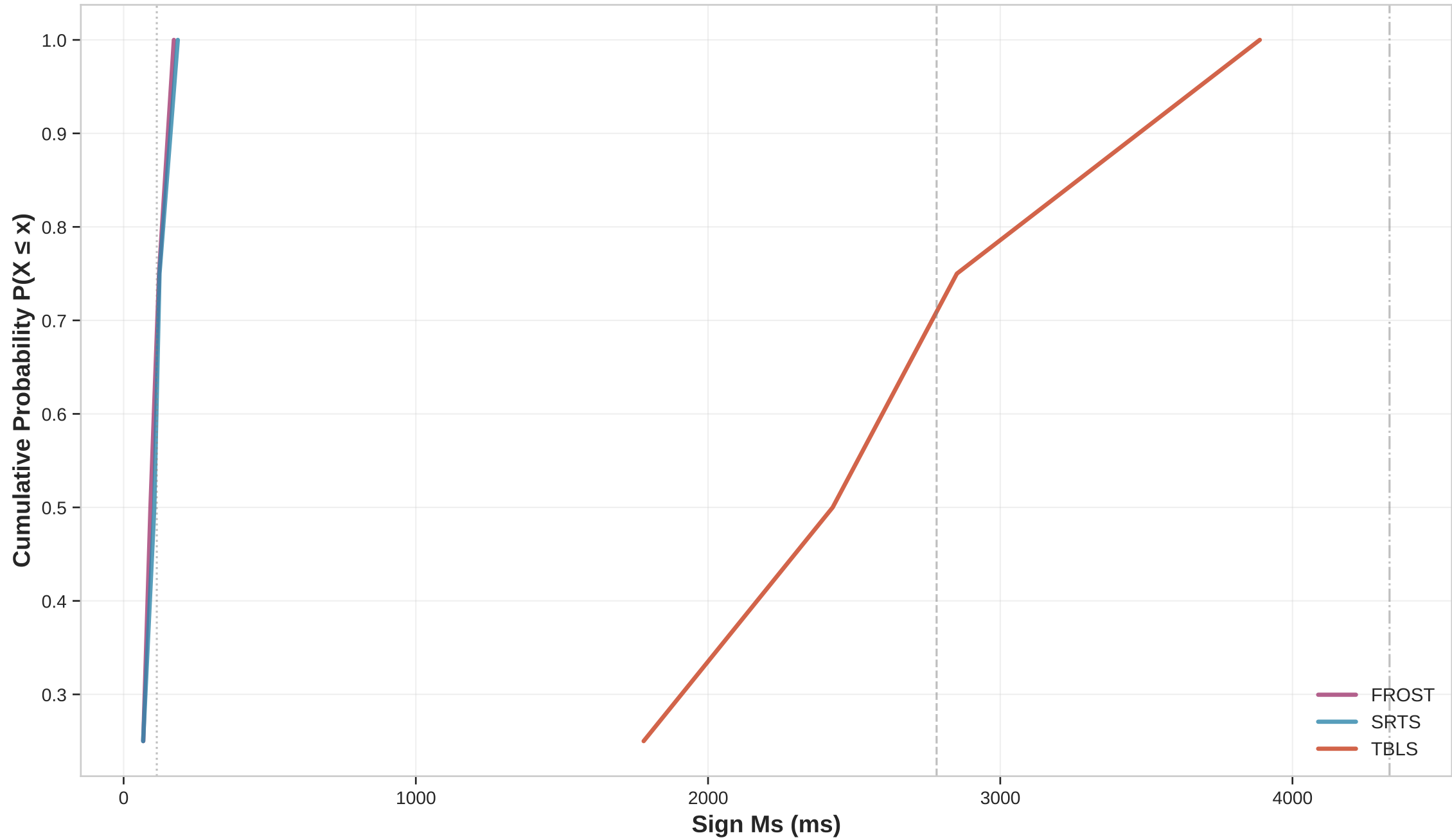
Time-to-Completion CDF (Packet Loss = 5.0%) (Shows tail latency and reliability)
