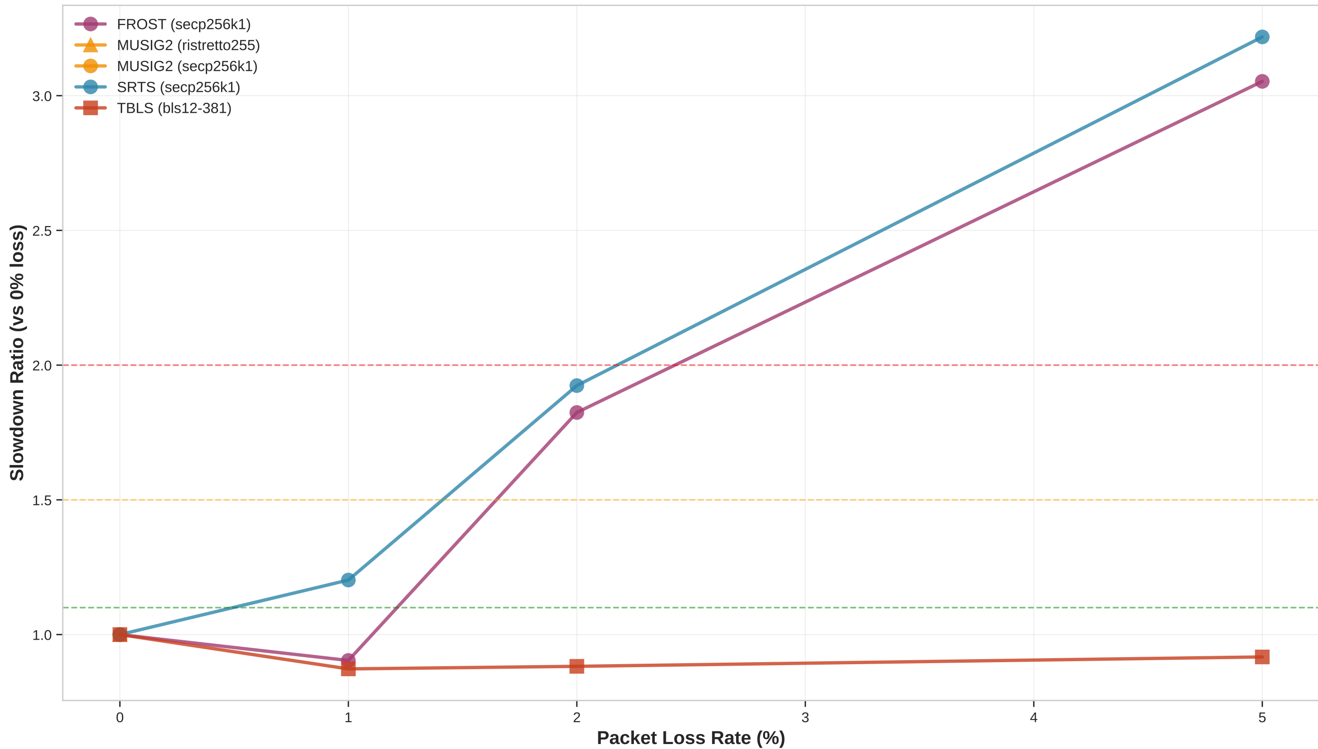
Performance Degradation Curve (Network Overhead vs Packet Loss) (Shows breaking point where schemes become unusable)
