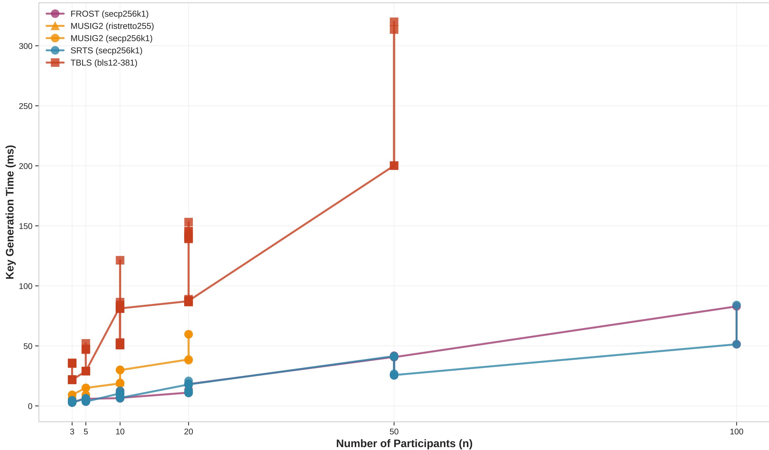
DKG Protocol Performance: Key Generation Time (One-time setup cost per swarm configuration)
