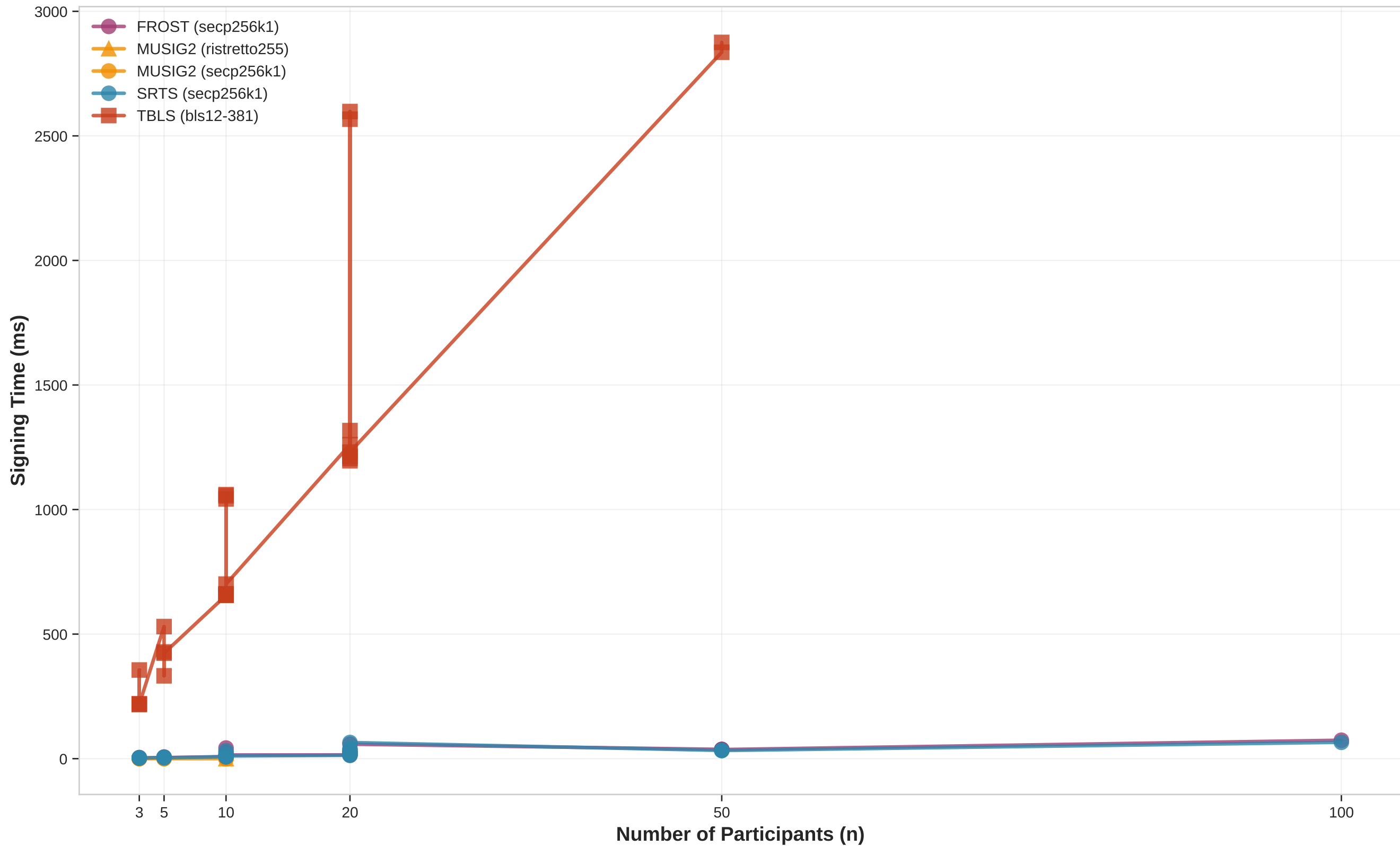
Threshold Signature Schemes: Signing Latency vs Swarm Size
