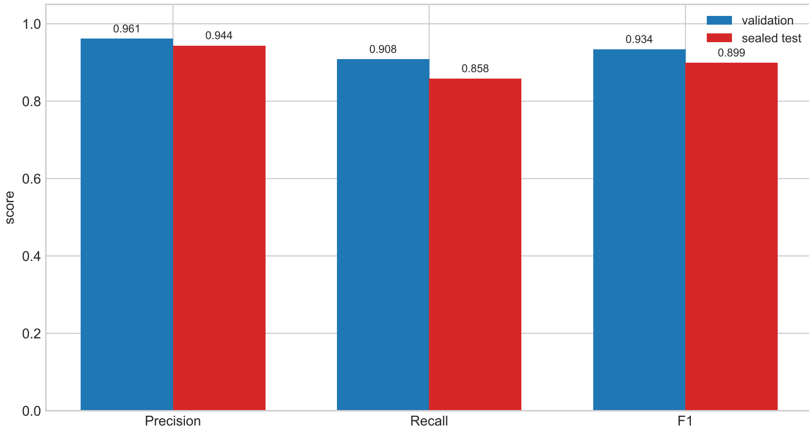
Validation vs Sealed-Test Operating Metrics at Threshold 0.999
