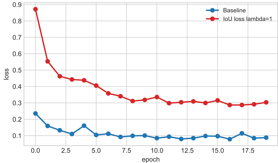
Validation Total Loss
