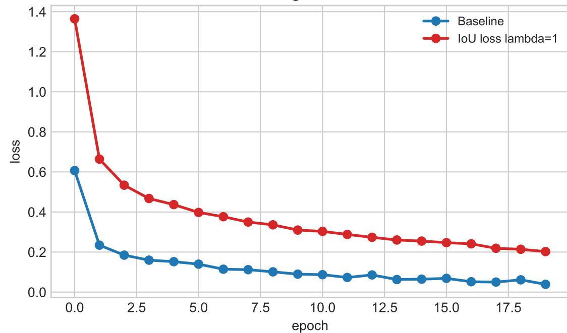
Training Total Loss
