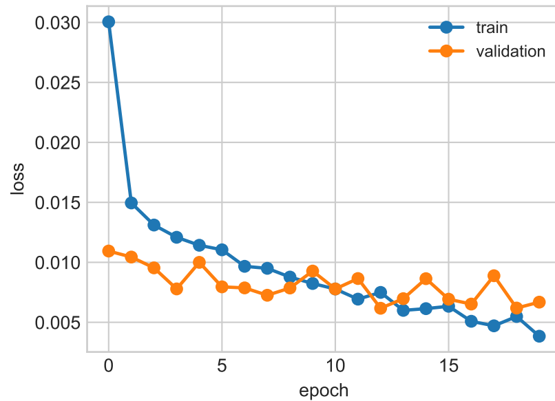
center regression
