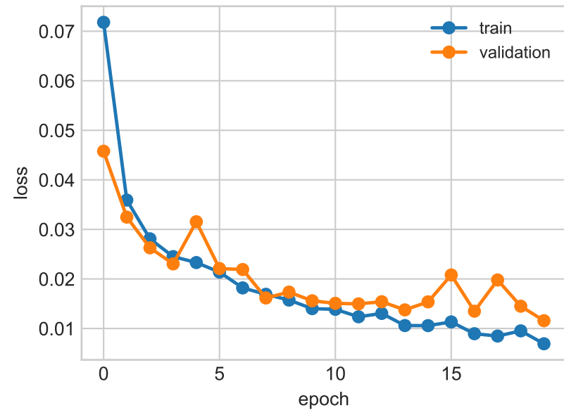
size regression
