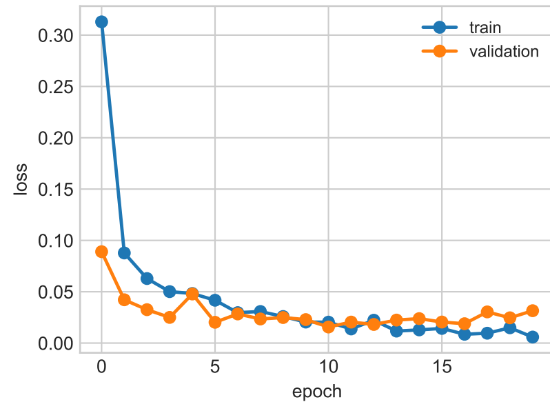
objectness
