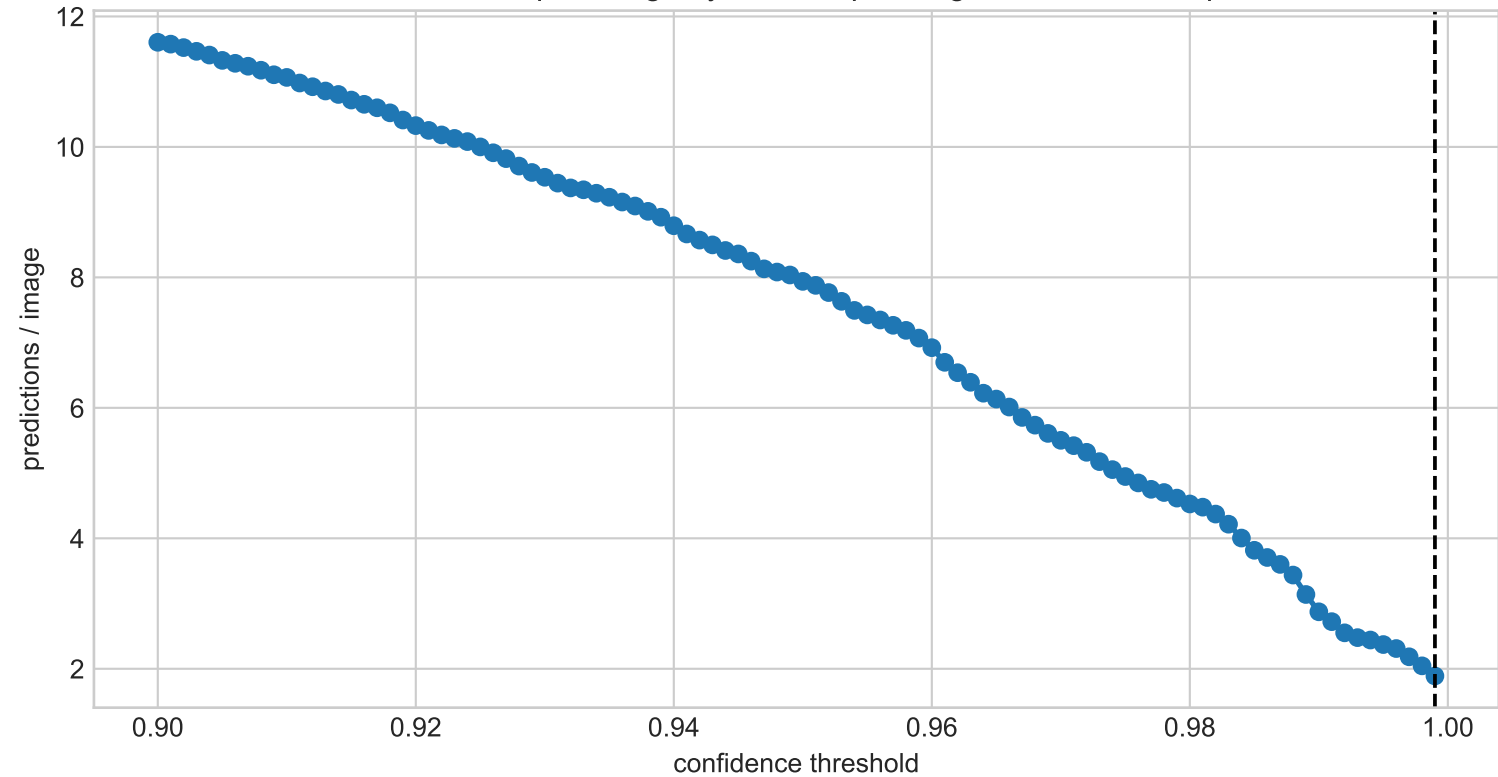
Predictions per Image by Broad Operating Threshold Sweep
