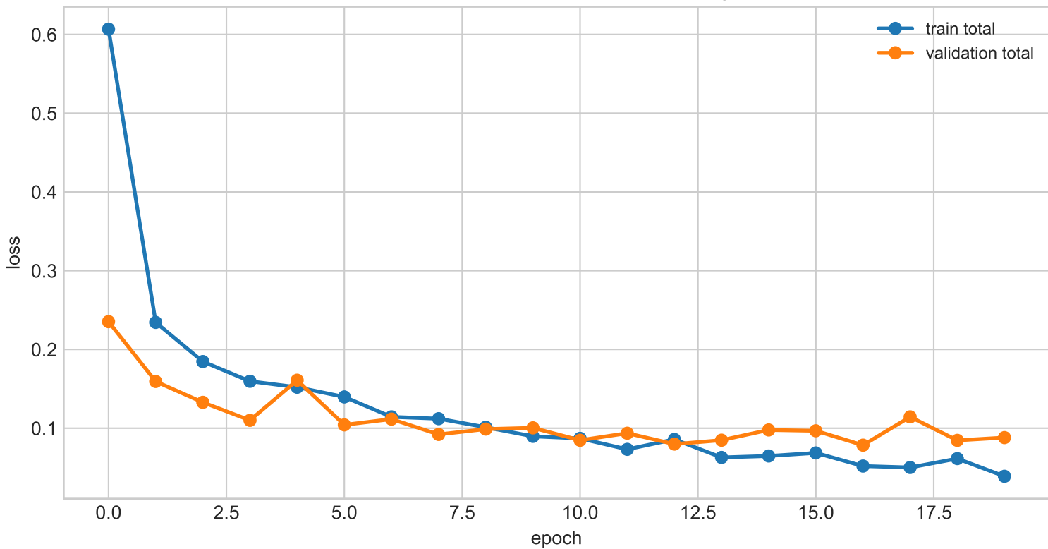
S8-CFD Total Loss Across Training
