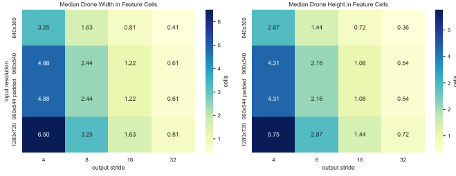
Fig. 1. Resolution and stride analysis used when choosing the 960×544 canvas and stride-8 prediction grid for small objects.
