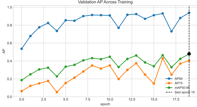
Fig. 2. Baseline validation AP curves. The validation-best checkpoint is selected by mAP50-95, not by operating F1.
