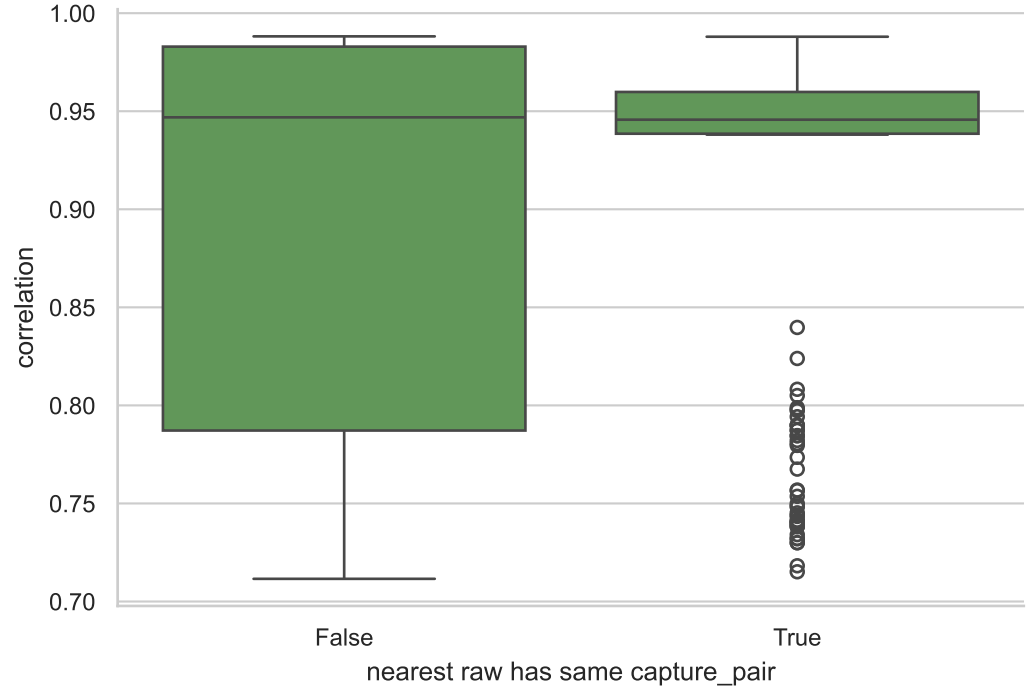
Nearest Similarity by Capture-Pair Match
