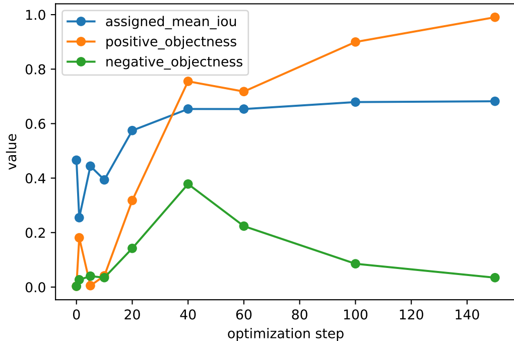
Tiny-Set Assigned-Cell Diagnostics
