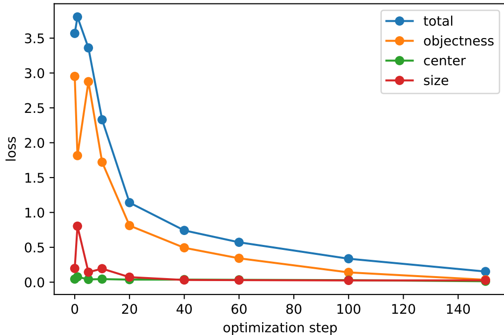
Tiny-Set Overfit Loss Diagnostic
