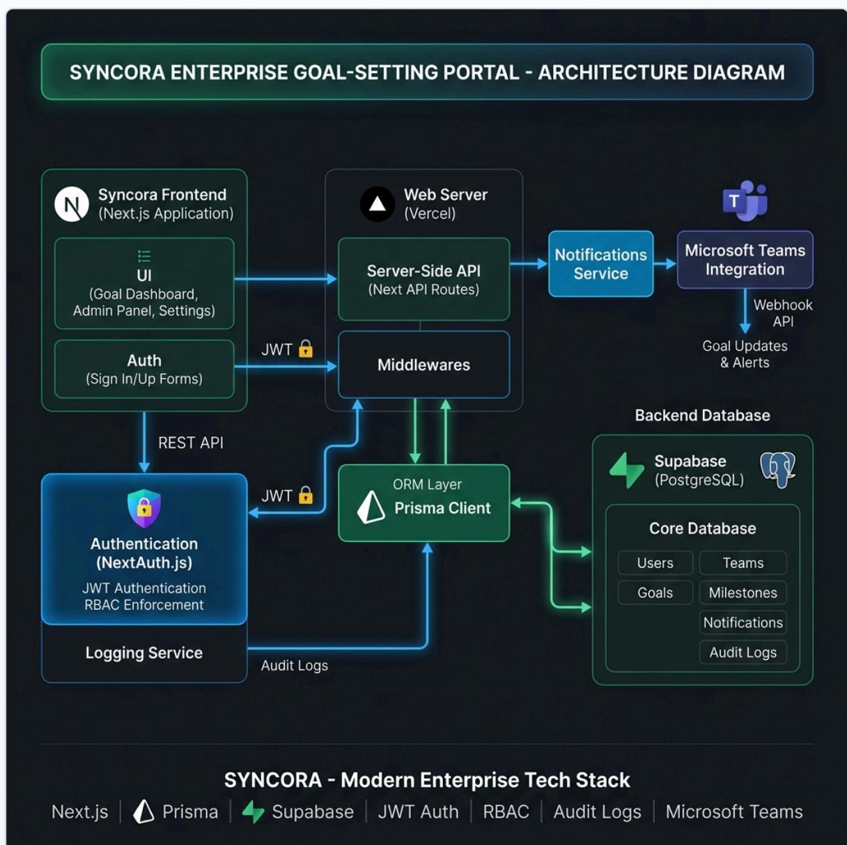
Figure 1: Cloud-Native Enterprise System Architecture
