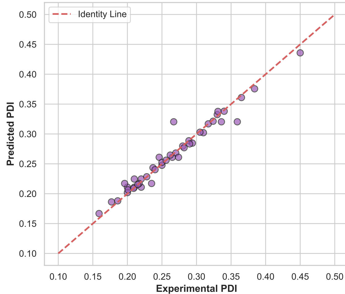
Chitosan PDI ( R^2 = 0.957 )
