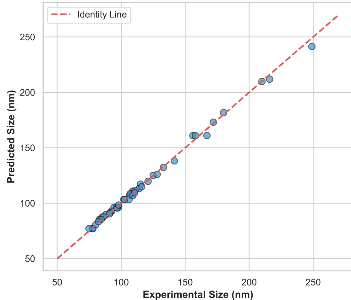
Chitosan Particle Size ( R^2 = 0.997 )
