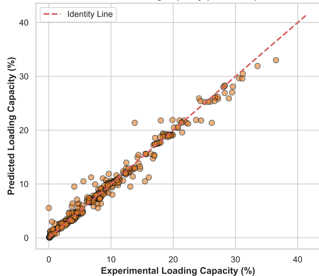
PLGA Loading Capacity ( R^2 = 0.977 )
