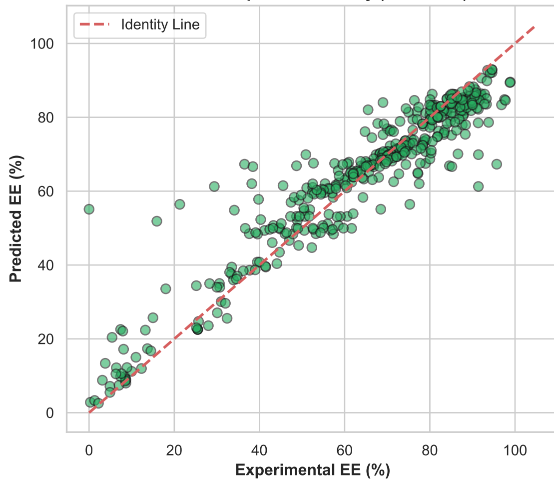
PLGA Entrapment Efficiency ( R^2 = 0.888 )
