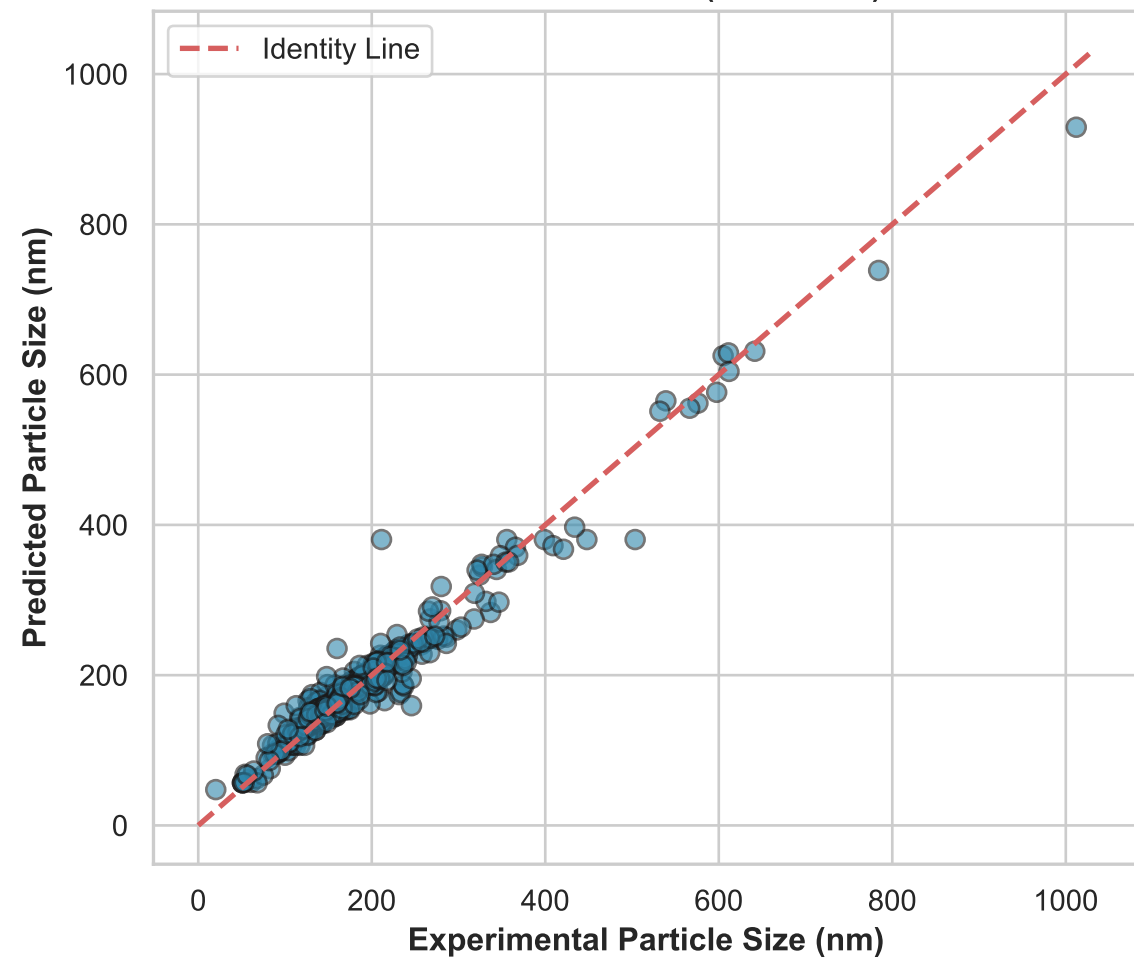
PLGA Particle Size ( R^2 = 0.959 )
