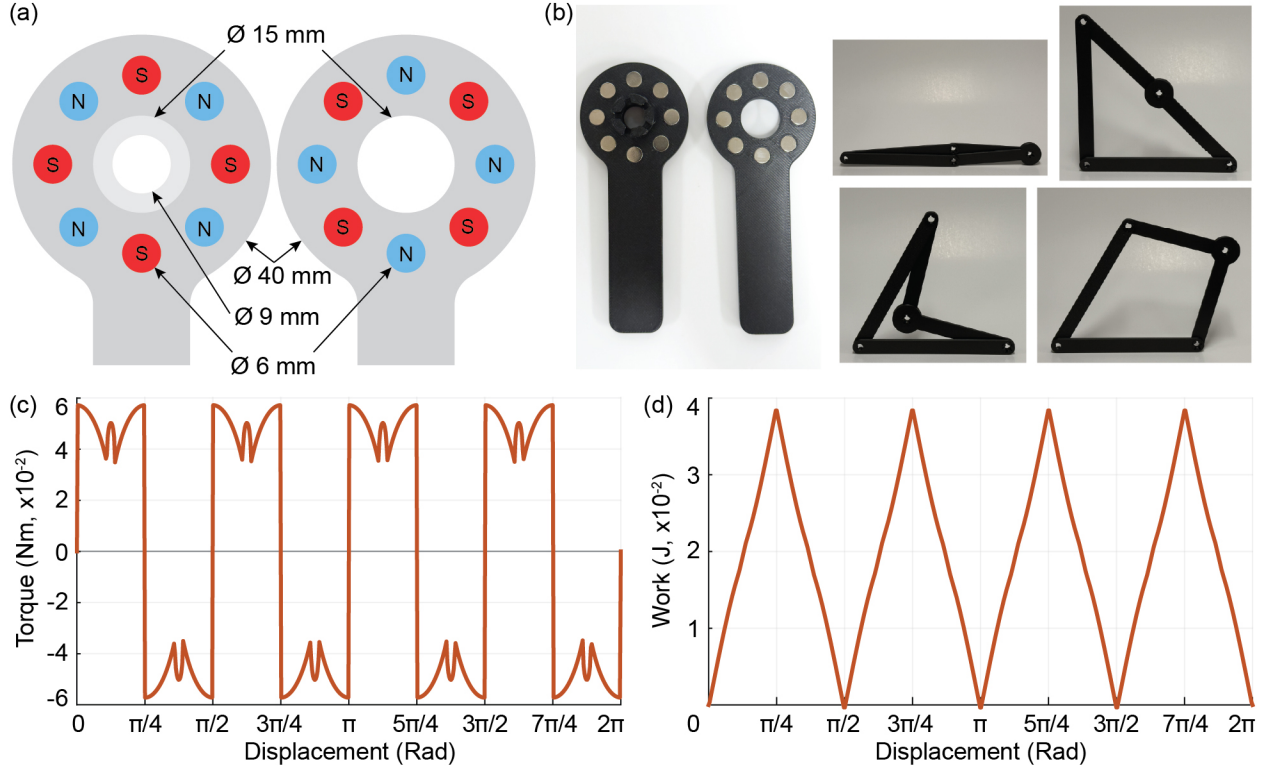
Figure 4.3: Magnetic multistable torsional hinge prototype. (a) Dimensions and magnet placement of the torsional hinge hub; (b) 3D printed and assemble prototye of a magnetic multistable hinge in a single unit truss; Simulated behavior of the magnetic multistable torsional hinge using a reduced-order magnetic interaction model: (c) Torque-displacement, and (d) Work-displacement response.
