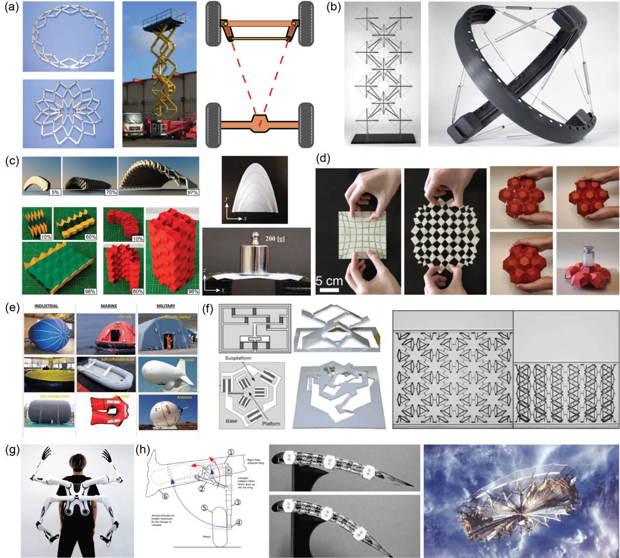
Figure 1.1: Examples of reconfigurable systems across engineering disciplines. (a) Bar-linked mechanisms: Hoberman linkage [1] (left, licensed under CC BY-NC-ND 3.0.), Scissor lift [2] (middle, licensed under CC BY-SA 2.0 Germany) and Ackermann steering linkage [3] (right, licensed under CC BY-SA 3.0); (b) Tensegrity structures: planar tensegrity mast [4] (left, adapted with permission from Sage Publications) and sperical tensegrity robot [5] (Copyright © 2016, IEEE); (c) Origami tubes for stiff columns, bridges and domes [6] (left) and curved-crease origami [7] (right, adapted with permission from Springer Nature); (d) Kirigami systems: planar auxetic kirigami [8] (left, adapted with permission from Springer Nature) and pop-up kirigami domes [9] (right, adapted with permission from Elsevier); (e) Membrane based inflatable systems [10] (licensed under CC BY-NC-ND 4.0); (f) Compliant mechanisms [11] (adapted with permission from Springer Nature) and multistable metamaterials [12] (licensed under CC BY 4.0); (g) Robotic arms [13] (licensed under CC BY 4.0); and (h) Aerospace systems: aircraft landing gear [14] (left), shape morphing wings [15] (middle, adapted with permission from Elsevier) and mesh reflector antenna deployed in orbit [16] (right, adapted with permission from Springer Nature).
