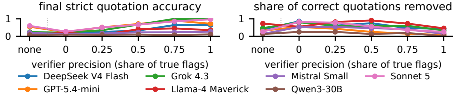
Figure 2. Verifier precision against what revision does. Left: final strict quotation accuracy. Right: share of accurate round-0 quotations that revision deleted, dequoted, or made inaccurate. Precision is the share of true feedback lines; the leftmost point is revision with no feedback.
