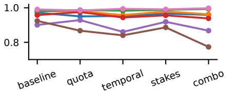
citation existence
