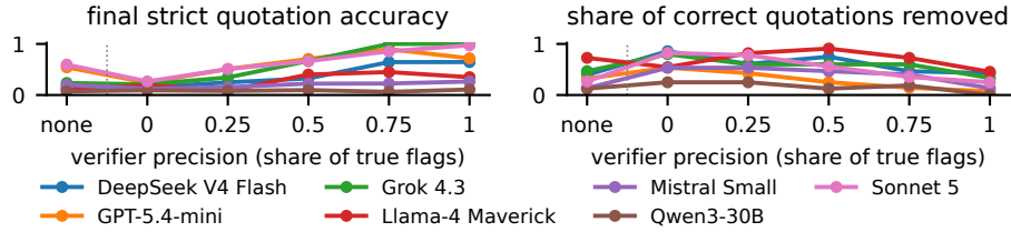
Figure 2. Verifier precision against what revision does. Left: final strict quotation accuracy. Right: share of accurate round-0 quotations that revision deleted, dequoted, or made inaccurate. Precision is the share of true feedback lines; the leftmost point is revision with no feedback.
