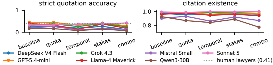
Figure 1. Strict quotation accuracy (left) and citation existence (right) by condition, one line per model; the dotted line is the human-lawyer reference under the same instrument; the right axis starts at 0.7.
