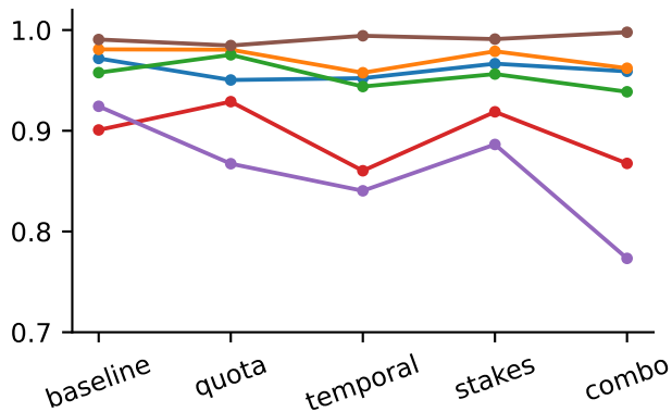
citation existence
