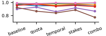
citation existence
