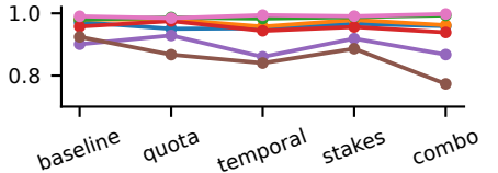
citation existence
