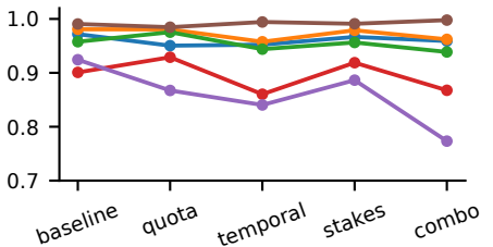
citation existence
