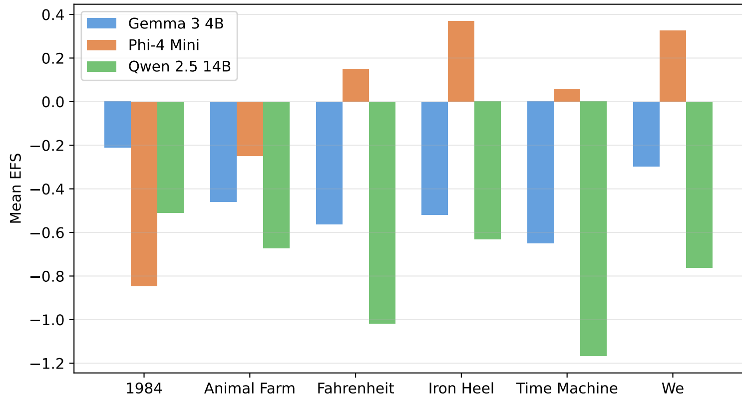
Mean EFS by Source Book and Model
