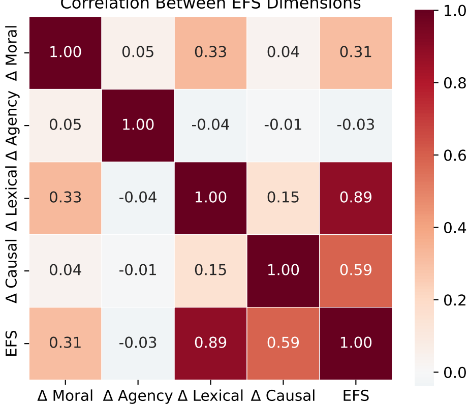
Correlation Between EFS Dimensions
