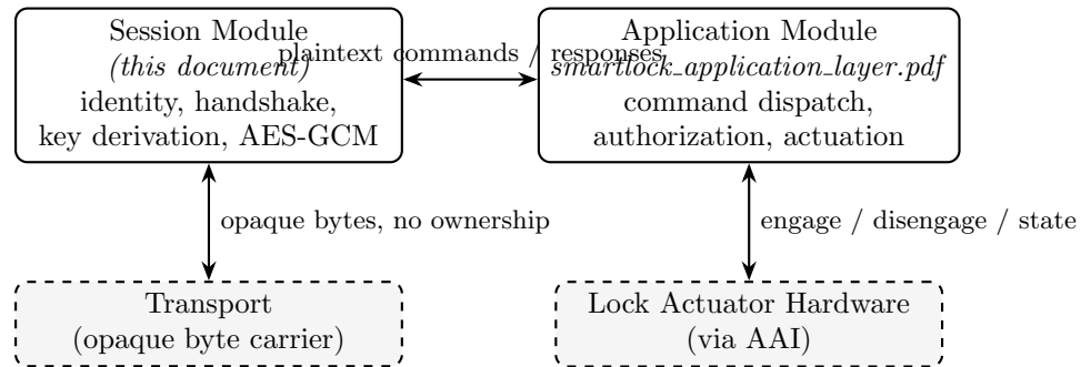
Figure 1: The session and application modules collaborate as peers. Each also has its own, independent external dependency (transport for this module, actuator hardware for the application module) that the other module never touches directly.
