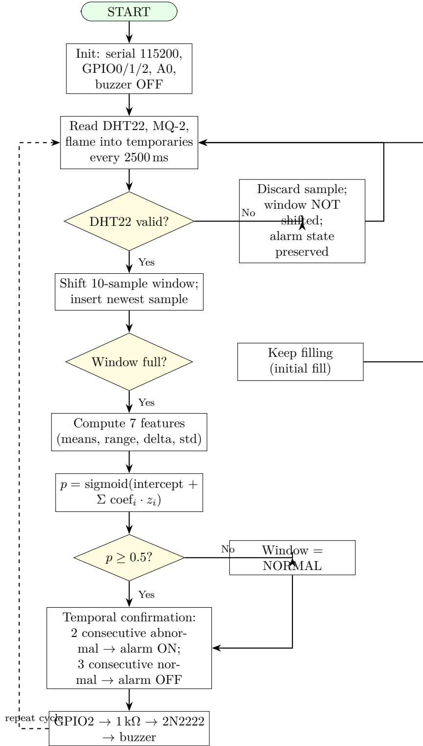
Figure 2: Firmware flowchart (one monitoring cycle).
