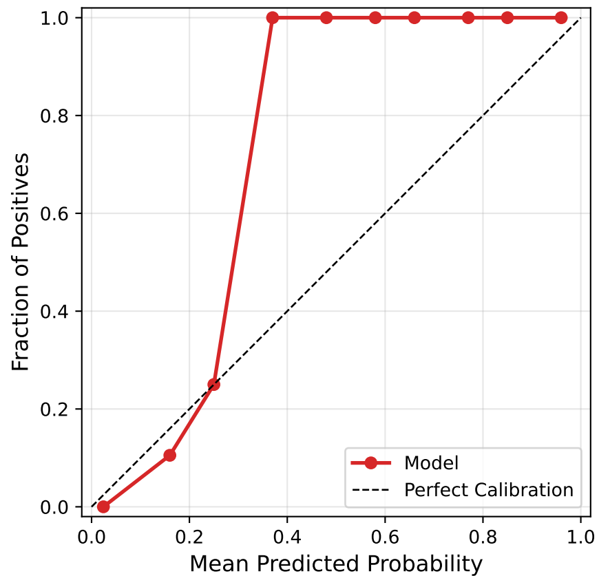
Mortality - Calibration Brier Score = 0.029
