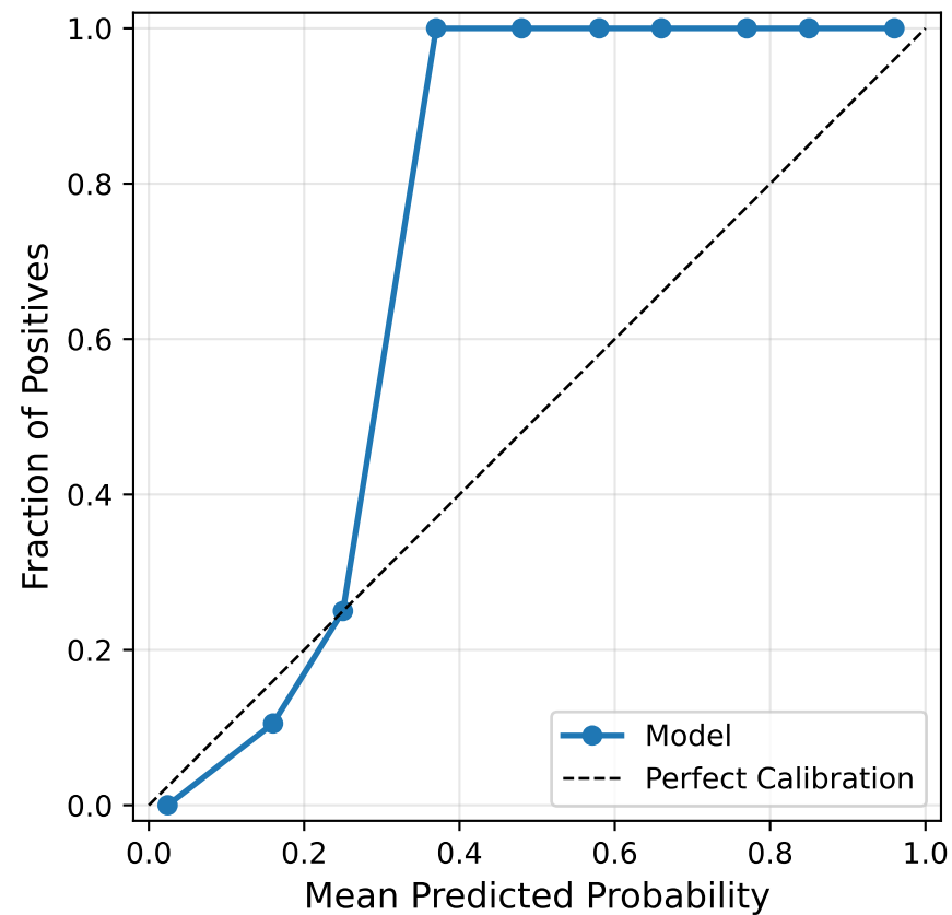
Cardiovascular - Calibration Brier Score = 0.029
