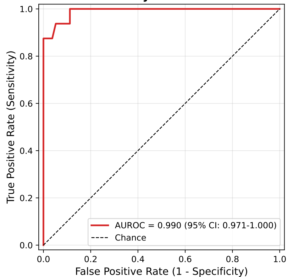
Mortality - ROC Curve
