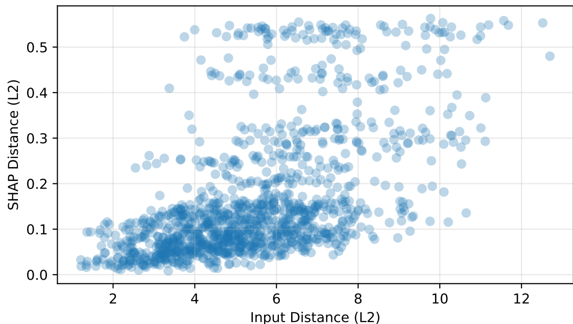
SHAP Stability Correlation: 0.561
