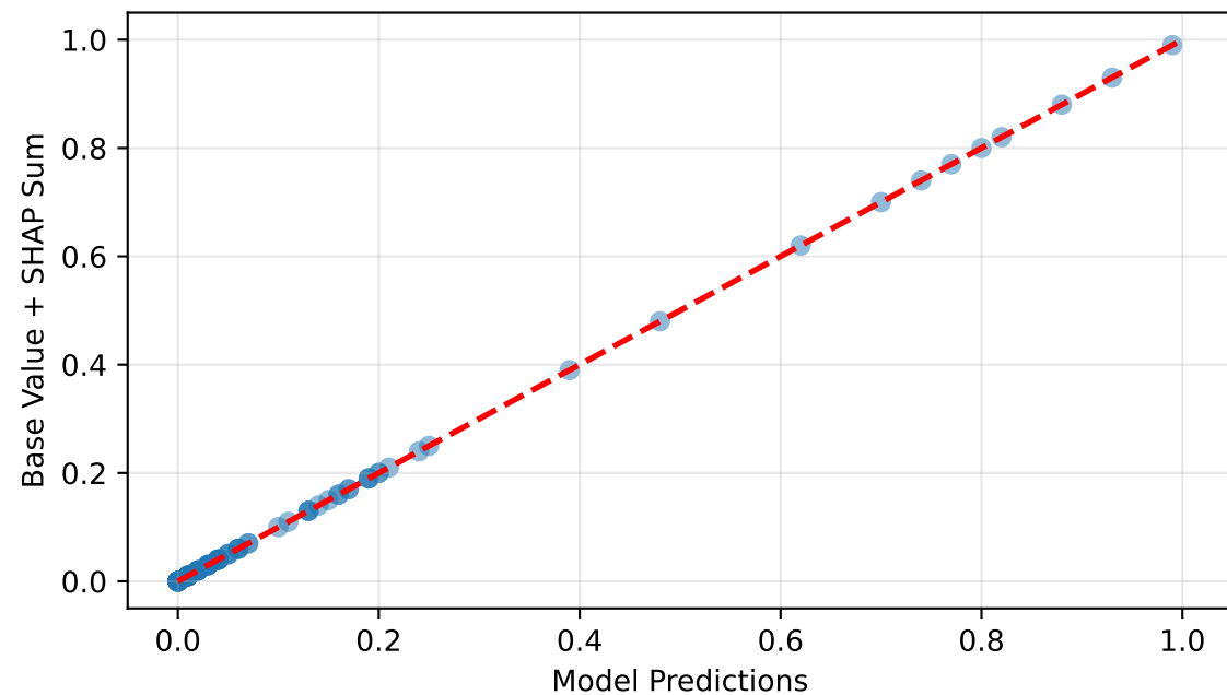
SHAP Additivity Check Mean Error: 0.000000
