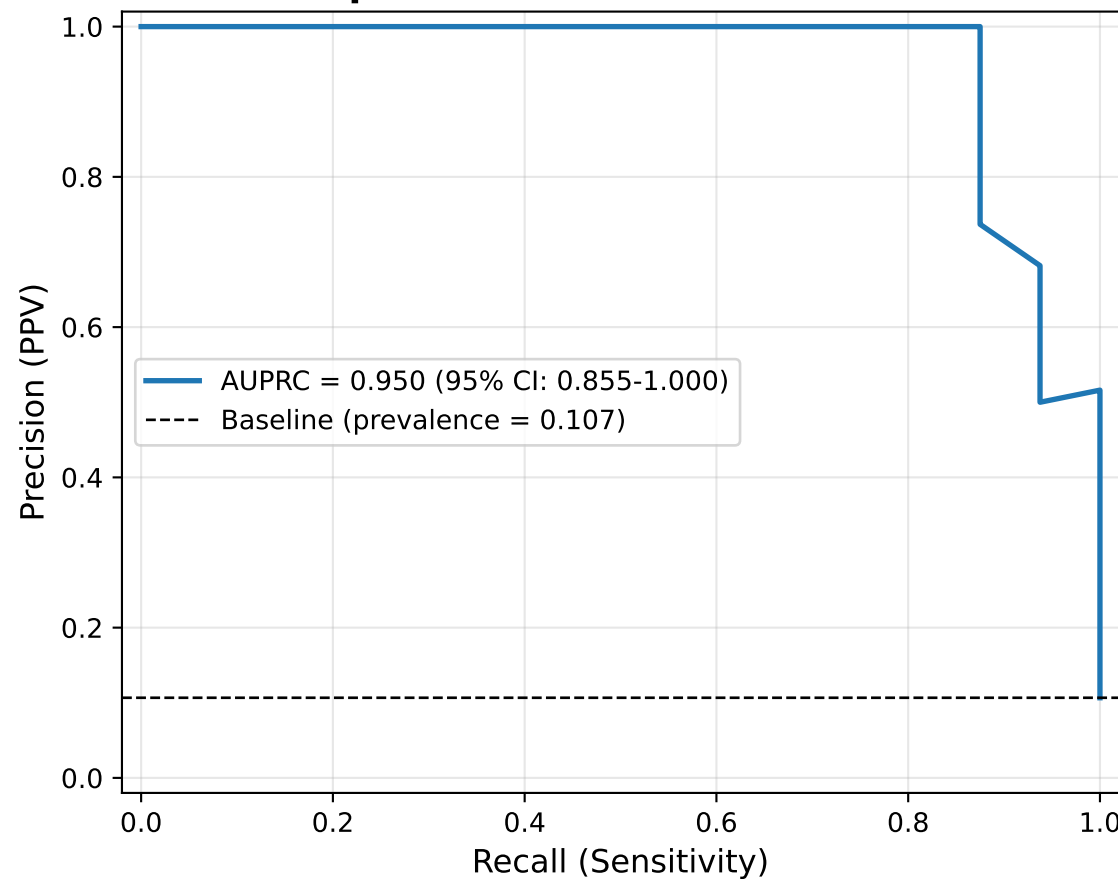
Cardiovascular - Precision-Recall Curve
