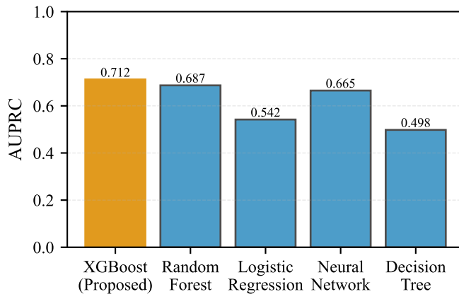
Model Performance Comparison Across Baselines
