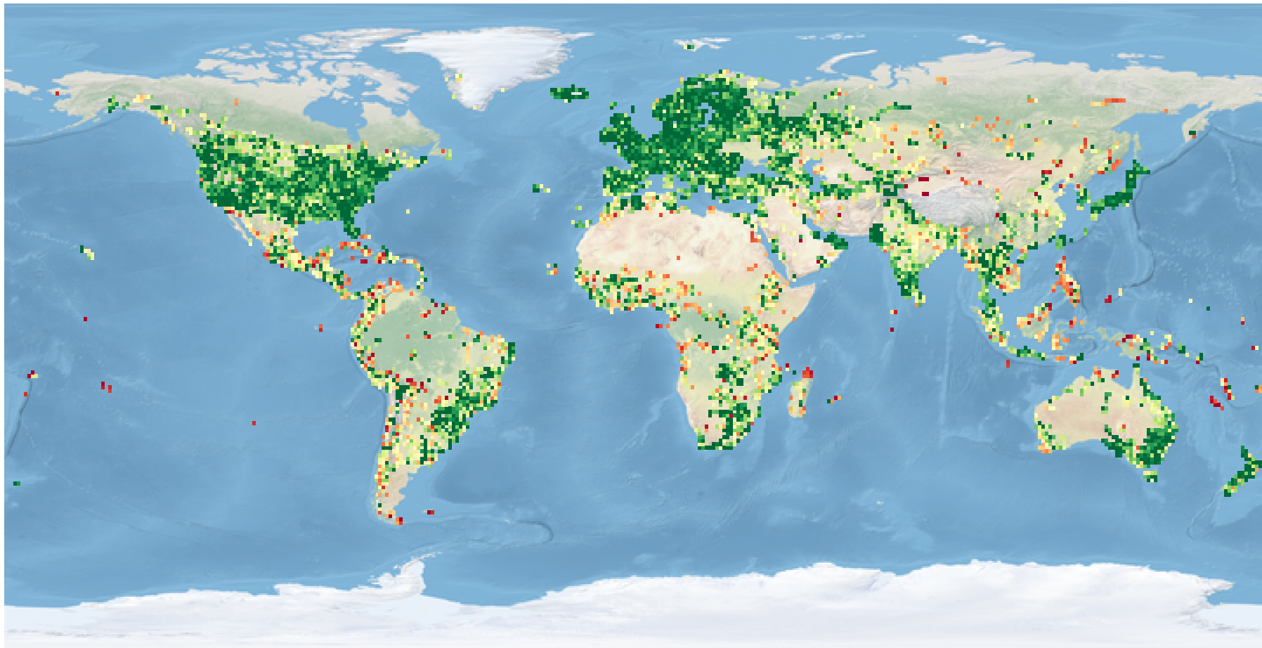
Mean Geolocation Error by Grid Cell ( 1^\circ \times 1^\circ ) HierLoc
