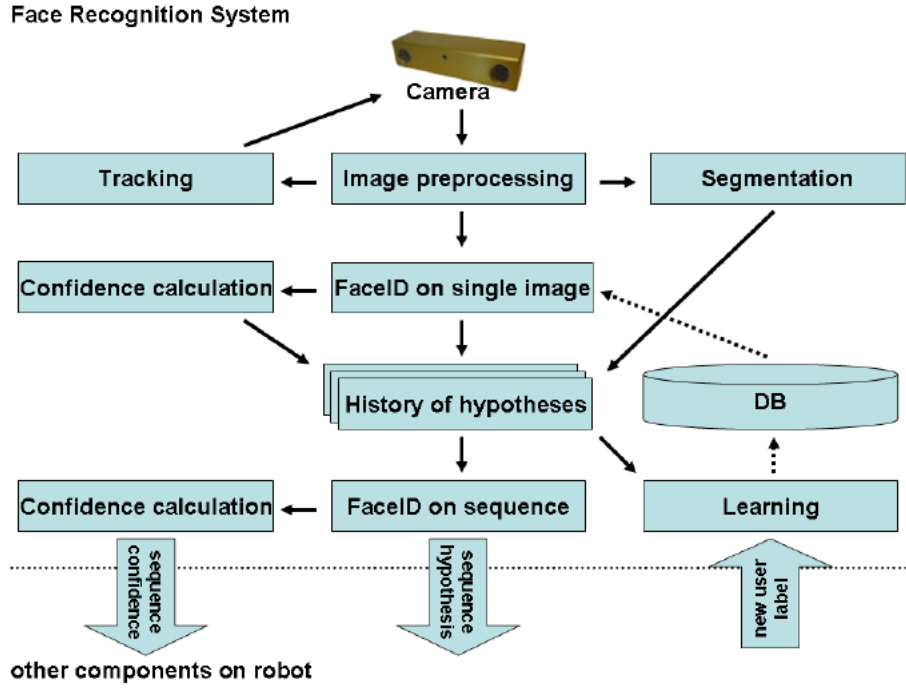
Figure 5.2: System architecture of face recognition system
