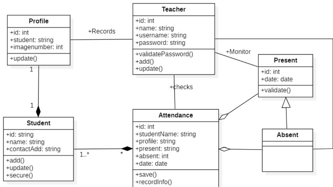
Figure 4.4: Class Diagram
