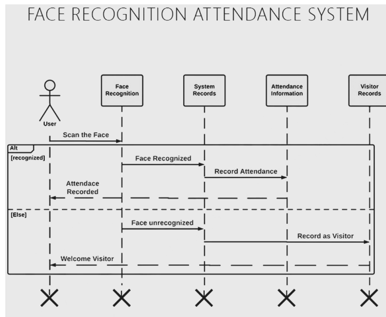
Figure 4.3: Sequence Diagram
