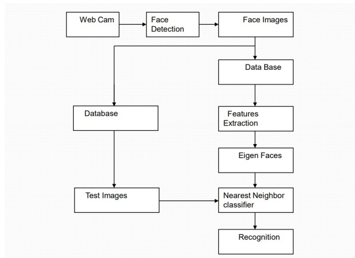
Figure 4.2: System Block Diagram
