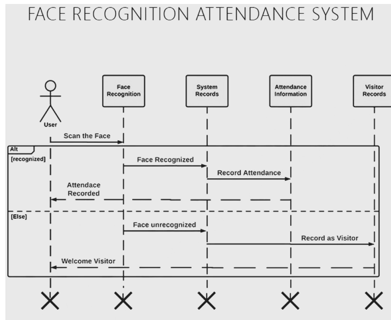
Figure 4.3: Sequence Diagram
