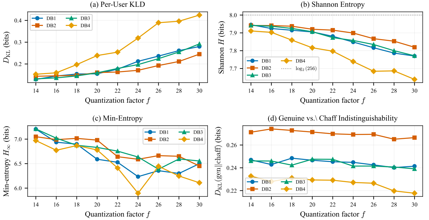
Fig. 15: Entropy analysis across quantization factors f \in [14, 30] . (a) Per-user KL divergence from uniform: all databases remain below 0.43 bits even at f = 30 . (b) Shannon entropy stays within 0.36 bits of the 8-bit theoretical maximum. (c) Min-entropy H_\infty \geq 5.9 bits guarantees worst-case unpredictability. (d) Genuine-vs-chaff KLD is nearly constant across factors ( \approx 0.24 bits), confirming that an adversary cannot distinguish genuine from chaff points regardless of the quantization granularity.
