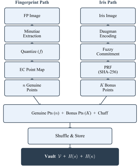
Fig. 3: IBFV enrollment pipeline. The fingerprint path produces genuine vault points via EC mapping onto Brainpool P256r1. The iris path extracts a stable key via fuzzy commitment, which seeds a PRF to derive K bonus polynomial points. All points are merged with chaff and shuffled into the final vault.
