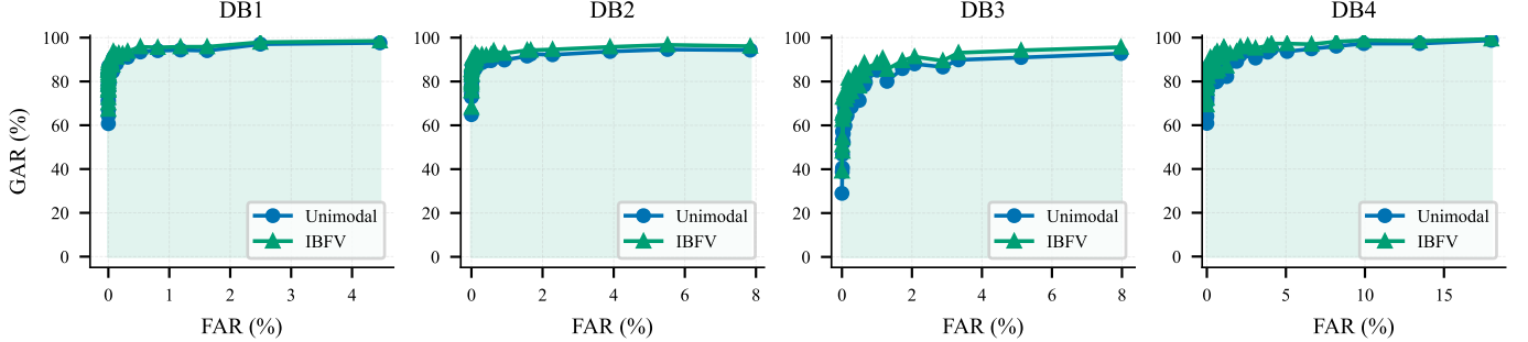
Fig. 11: ROC curves for Setup 2. The shaded area under the IBFV curve illustrates the AUC improvement over the unimodal baseline.
