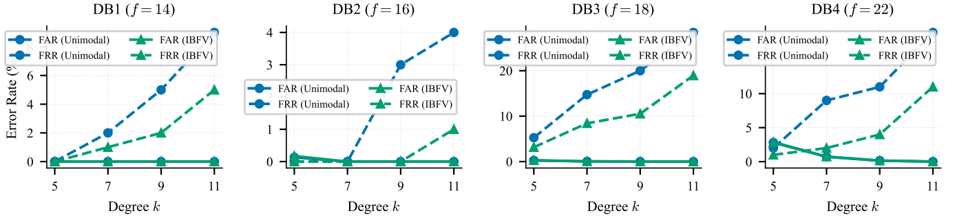
Fig. 9: FAR/FRR crossover curves (Setup 1, best factor per database). The intersection of FAR and FRR defines the EER operating point. IBFV shifts the FRR curve downward without increasing FAR.
