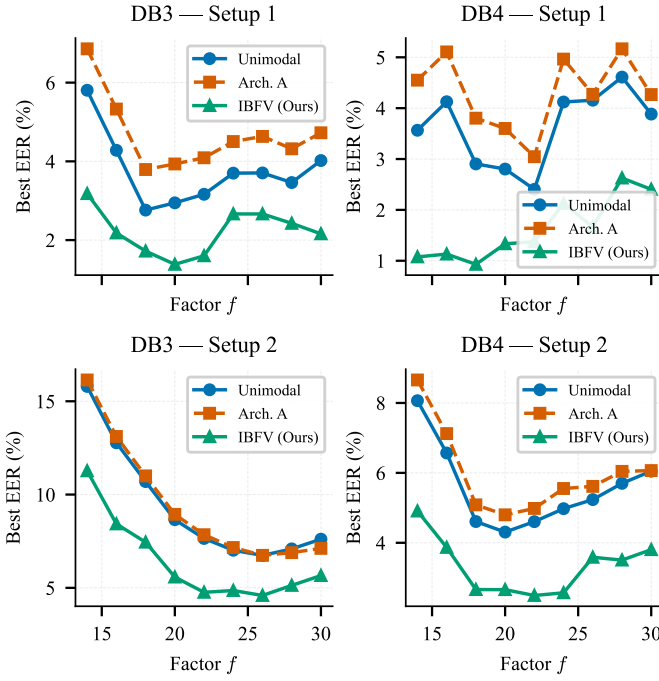
Fig. 7: EER vs. quantization factor f (best over degrees k ) for DB3 and DB4 under both setups. IBFV consistently lies below the unimodal baseline and far below Architecture A at every operating point.
