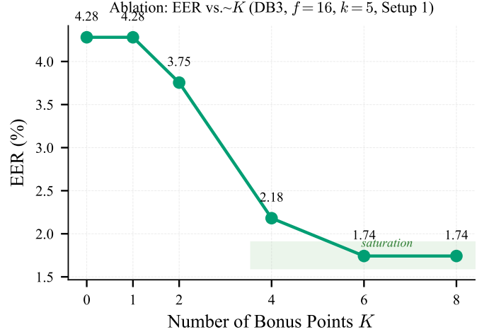
Fig. 16: Ablation study: EER (%) vs. number of iris-derived bonus points K on DB3 ( f = 16 , k = 5 , Setup 1). EER decreases monotonically until saturation at K = 6 .
