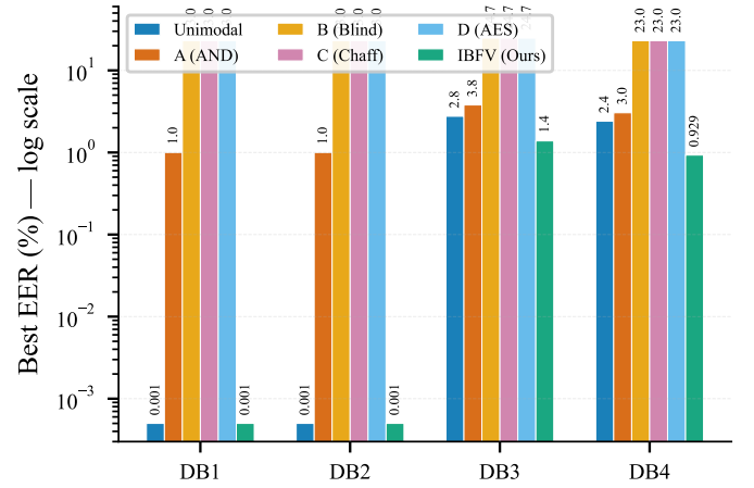
Fig. 6: Best EER comparison across all architectures (Setup 1). Architectures A–D all degrade performance relative to the unimodal baseline; only IBFV improves it. Note the log scale on the y-axis.
