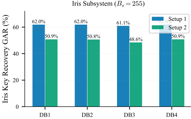
Fig. 14: Iris key recovery GAR by database and setup at B_s = 255 . Impostor FAR is \sim 0.10\% (Setup 1).
