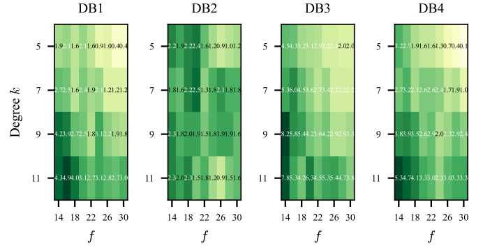
Fig. 8: \Delta EER (Unimodal – IBFV) in percentage points across all (f, k) configurations for Setup 2. All values are \geq 0 , confirming zero violations of the monotonicity guarantee.
