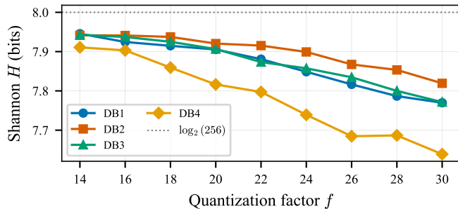
(b) Shannon Entropy
