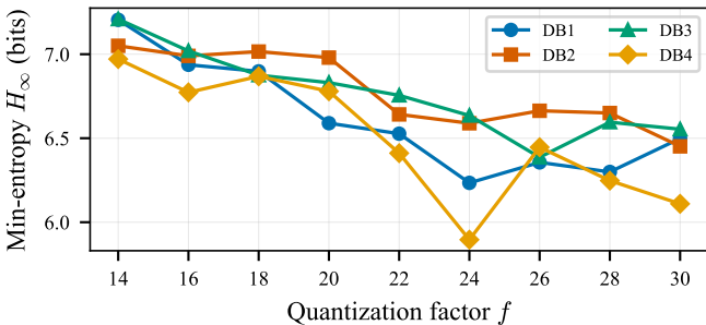
(c) Min-Entropy
